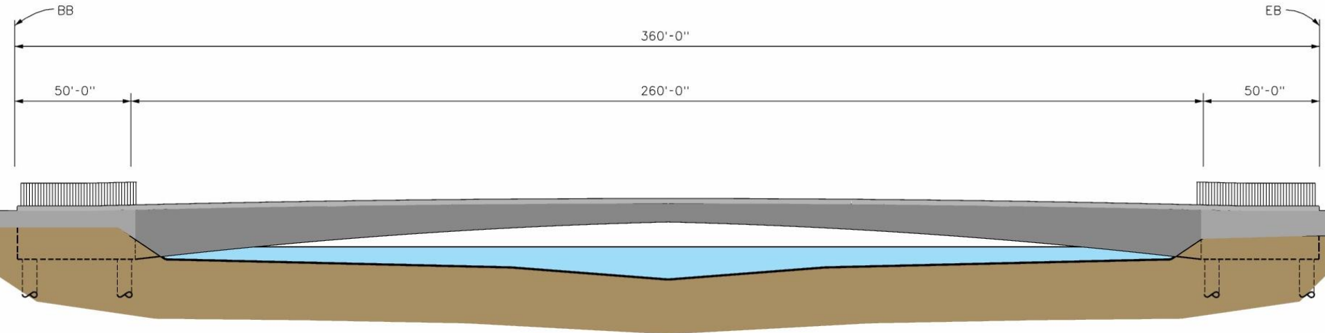
ELEVATION 1" = 20'
